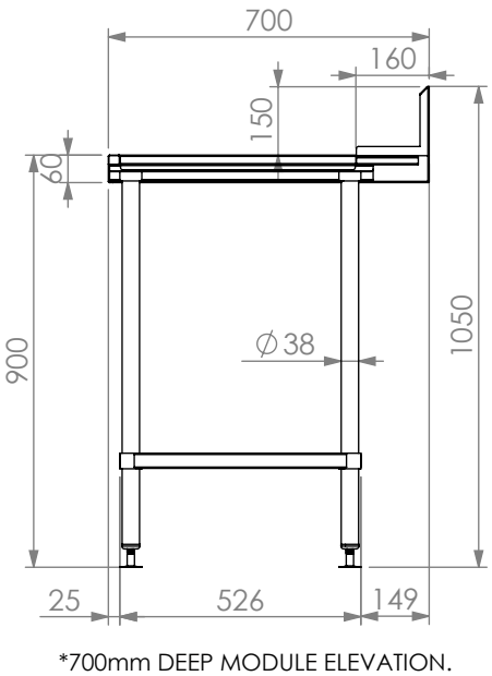
*700mm DEEP MODULE ELEVATION.
