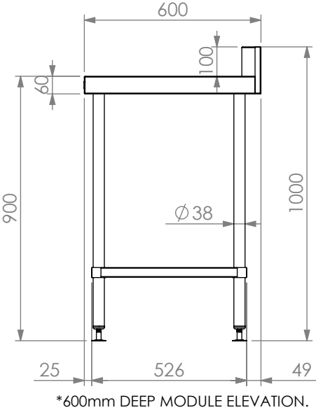
*600mm DEEP MODULE ELEVATION.
